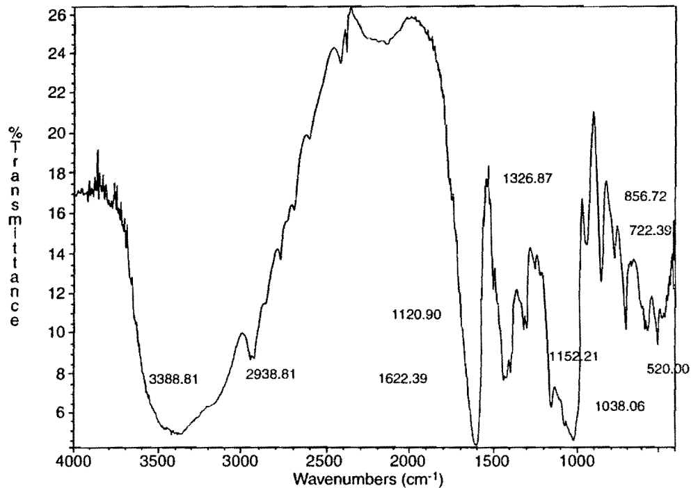
FIGURE 1 IR spectrum of Na-PCMS.
